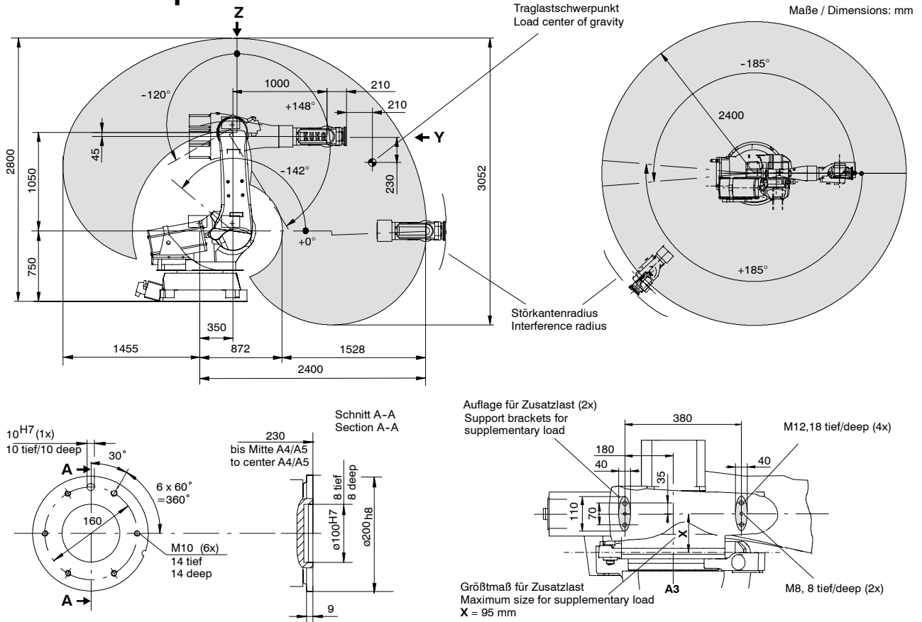
“Y” Anbaufansch A 6 Mounting flange A 6
